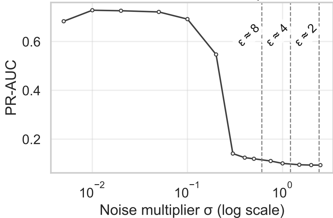
WUSTL Strict fixed-noise sweep: PR-AUC
